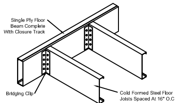
○ Floor Joist To Beam Connection
