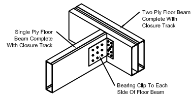
○ Floor Beam To Floor Beam Connection
