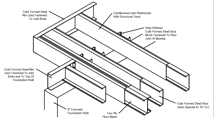
○ Cantilevered Floor Detail
