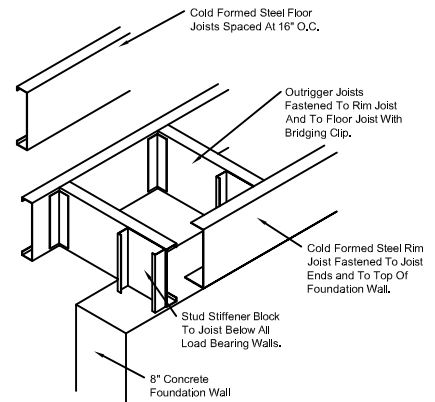
○ Floor Joist Outrigger Detail
