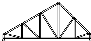
Dual Pitch Truss
