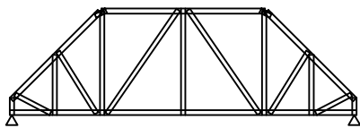
Hip Truss
