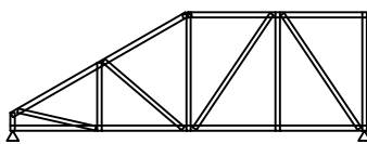
Half Hip Truss
